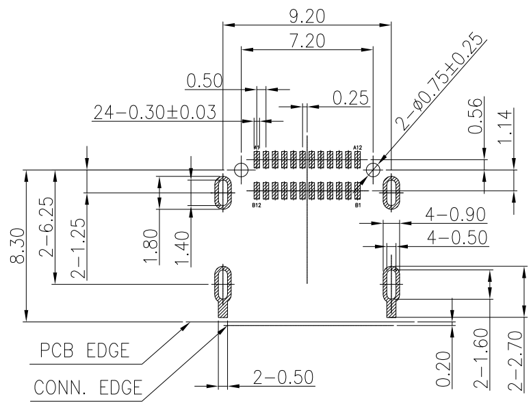
RECOMMENDED P.C.B LAYOUT (TOP VIEW) PCB THICKNESS: 1.00MM DEFAULT TOLERANCE ±0.05
