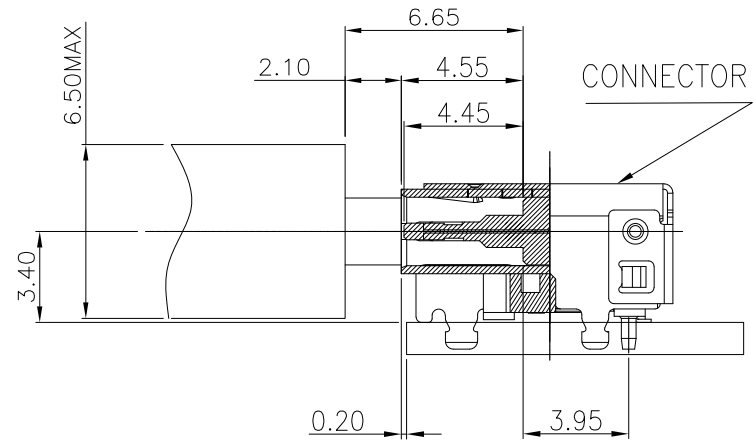
RECOMMENDED METHOD OF MATE SCALE: 1:1
