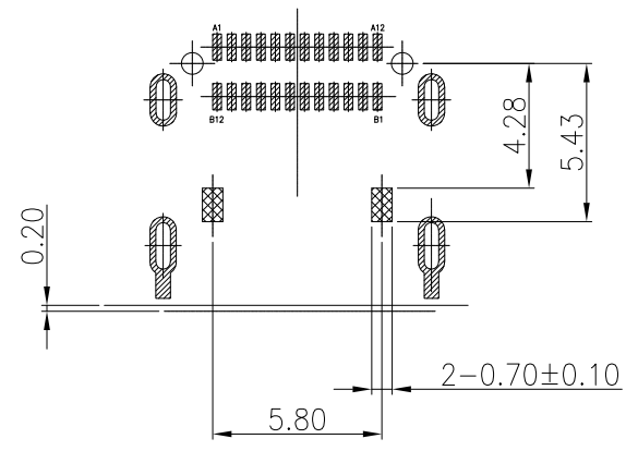
RECOMMENDED CONTACTOR EDGE COMPONENT SIDE: TOP VIEW ▨ STAND OFF AREA ▩ PAD AREA
